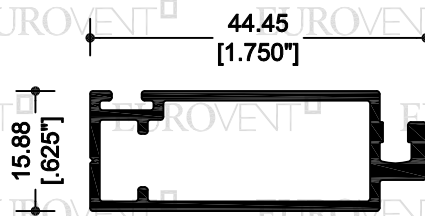
18930 MOSQUITERO
